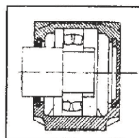
One End Cover & One V Ring Seals : Type ATA
