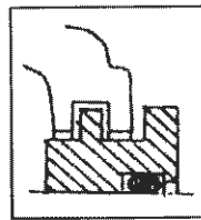
Type - S unsplit TSNA...S (2 Labyrinth Collars with rubber o' Cords)
