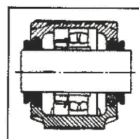
Housing with two labyrinth Seals : Type TS
