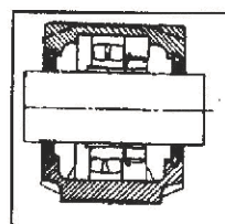
Housing with two V Ring : Type TA
