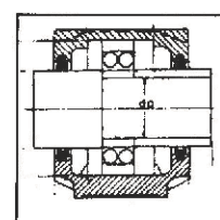
Housing with double Lip-Seals : Type TG
